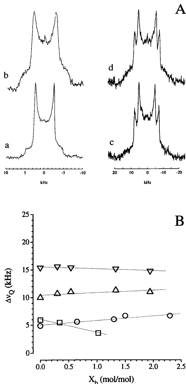
FIGURE 3 Deuterium NMR studies of deuterium-labeled 1-palmitoyl-2-oleoyl- sn -glycero-3-phosphocholine (POPC) in mixture with octyl- \beta -D-glucopyranoside (OG). The lipid headgroup region. (A) {}^2\text{H} -NMR spectra of multilayered lipid dispersions. The two lower spectra (a, c) correspond to pure lipid systems. The two upper spectra (b, d) correspond to lipid in mixture with OG. The specifics are: (a) \beta -CD 2 -POPC (pure lipid), \Delta\nu_Q = 4.9 kHz. (b) \beta -CD 2 -POPC plus OG, X_b = 1.3 , \Delta\nu_Q = 6.0 kHz. (c) POPC deuterated at the C-2 segment of the oleic acyl chain (2'-D 2 POPC) (pure lipid), \Delta\nu_{Q,1} = 15.4 kHz, \Delta\nu_{Q,2} = 10.0 kHz. (d) 2'-D 2 POPC plus OG, X_b = 0.54 , \Delta\nu_{Q,1} = 15.4 kHz, \Delta\nu_{Q,2} = 11.0 kHz. Deuterium frequency 61.4 MHz, 8000 transients, T = 28^\circ\text{C} . (B) Variation of the quadrupole splittings, \Delta\nu_Q , of deuterated POPC lipids with X_b , the amount of bound OG. \Delta , \nabla , 2'-D 2 POPC. \square , \alpha -CD 2 -POPC. \circ , \beta -CD 2 -POPC.
