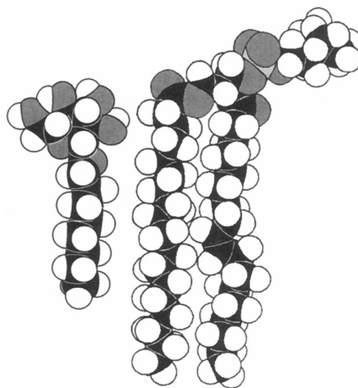
FIGURE 8 Diagram (to scale) of octyl- \beta -D-glucopyranoside (OG, left) and 1-palmitoyl-2-oleoyl- sn -glycero-3-phosphocholine (POPC, right), showing the approximate location of the two molecules in the membrane, as suggested by the monolayer and ^2\text{H} -NMR measurements.
