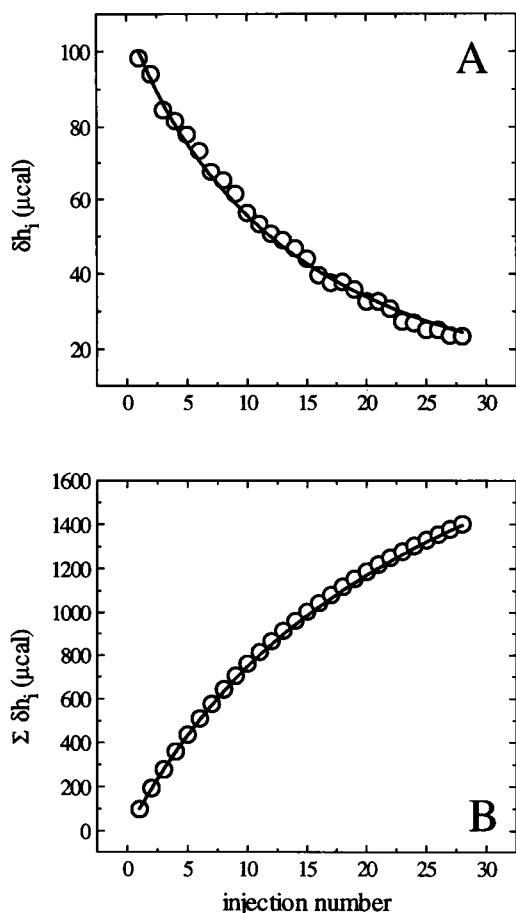
FIGURE 6 Simulation of the experimental data shown in Fig. 1 with the partition model using K = 115 \text{ M}^{-1} and \Delta H_D^0 = 1.25 \text{ kcal/mol} . The experimental data are shown as open circles. The solid line represents the theoretical simulation. (A) Individual titration peaks. (B) Cumulative heat of reaction.
